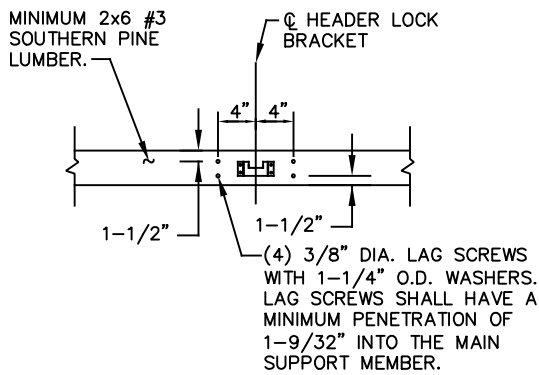
DETAIL 3 WOOD SUPPORT STRUCTURE NOTE: MAXIMUM DESIGN LOAD CAPACITY OF 2430 LBS.
